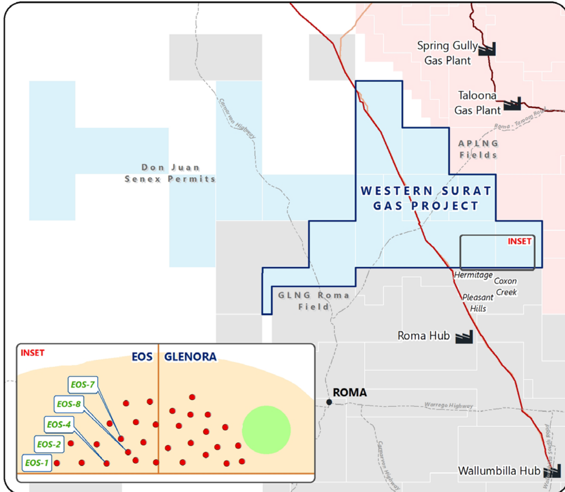
Figure 1: Surat Basin Senex drilling activity for July 2017
